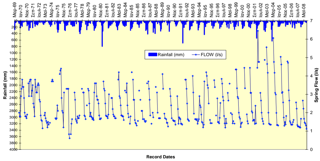
s9-6-3-12 - ΛΟΥΜΑΤΑ ΤΟΥ ΑΕΤΟΥ "Α" - Troodos PWD Meteorological Station (Station 270)
