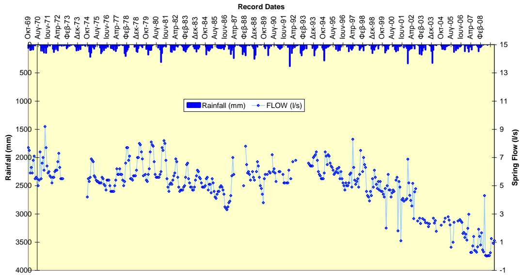
s3-3-1-80 - ΑΥΙΟΣ ΝΙΚΟΛΑΟΣ Α+Β - Kakopetria Meteorological Station (EL. School) (Station 291)
