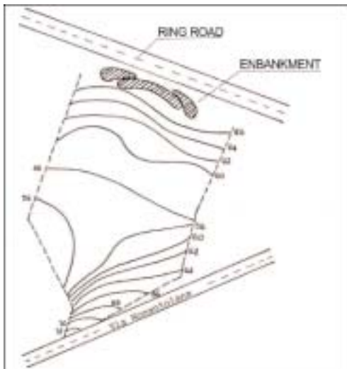
Figure 1: Noise contour map at 10 m above the ground in the Torrenova area
