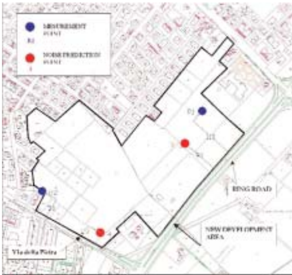
Figure 4: Plan of Via della Pietra residential area
