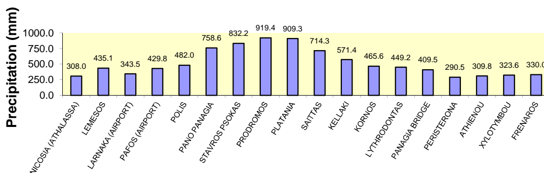
Normal Precipitation (mm) for main Meteorological Stations
